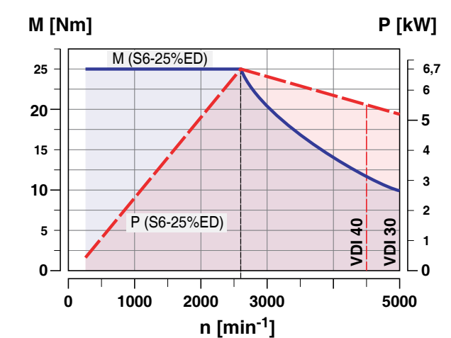
Tool turret motor characteristics for driven tools
