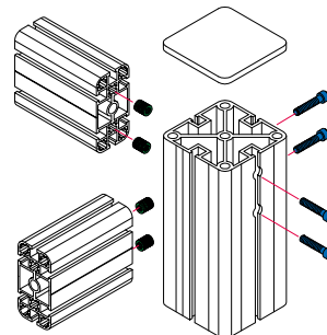
Example PS 80 with PL 80
