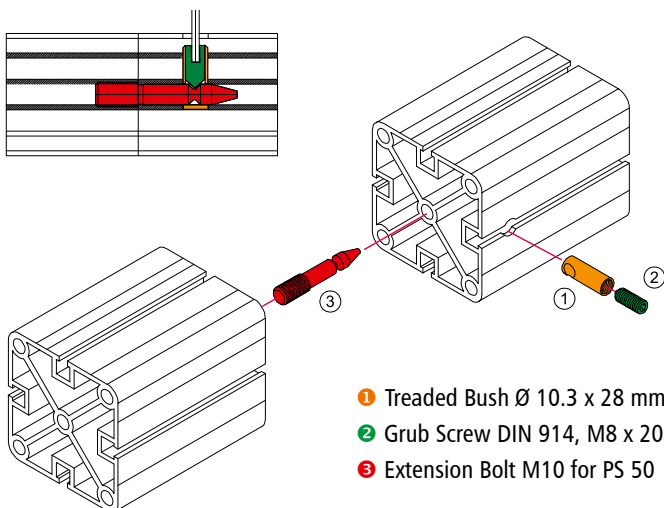
Example Profile snaplock extension for PS 50
